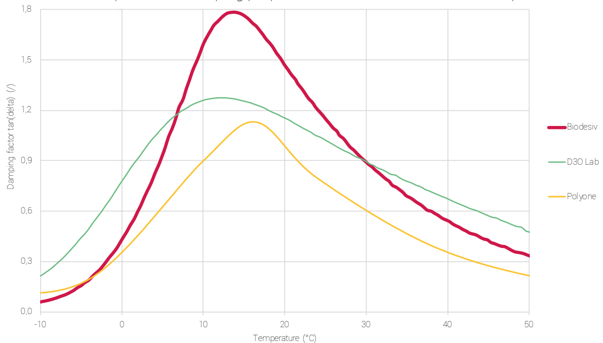
Comparison of damping properties of Biodesiv material and competitors
